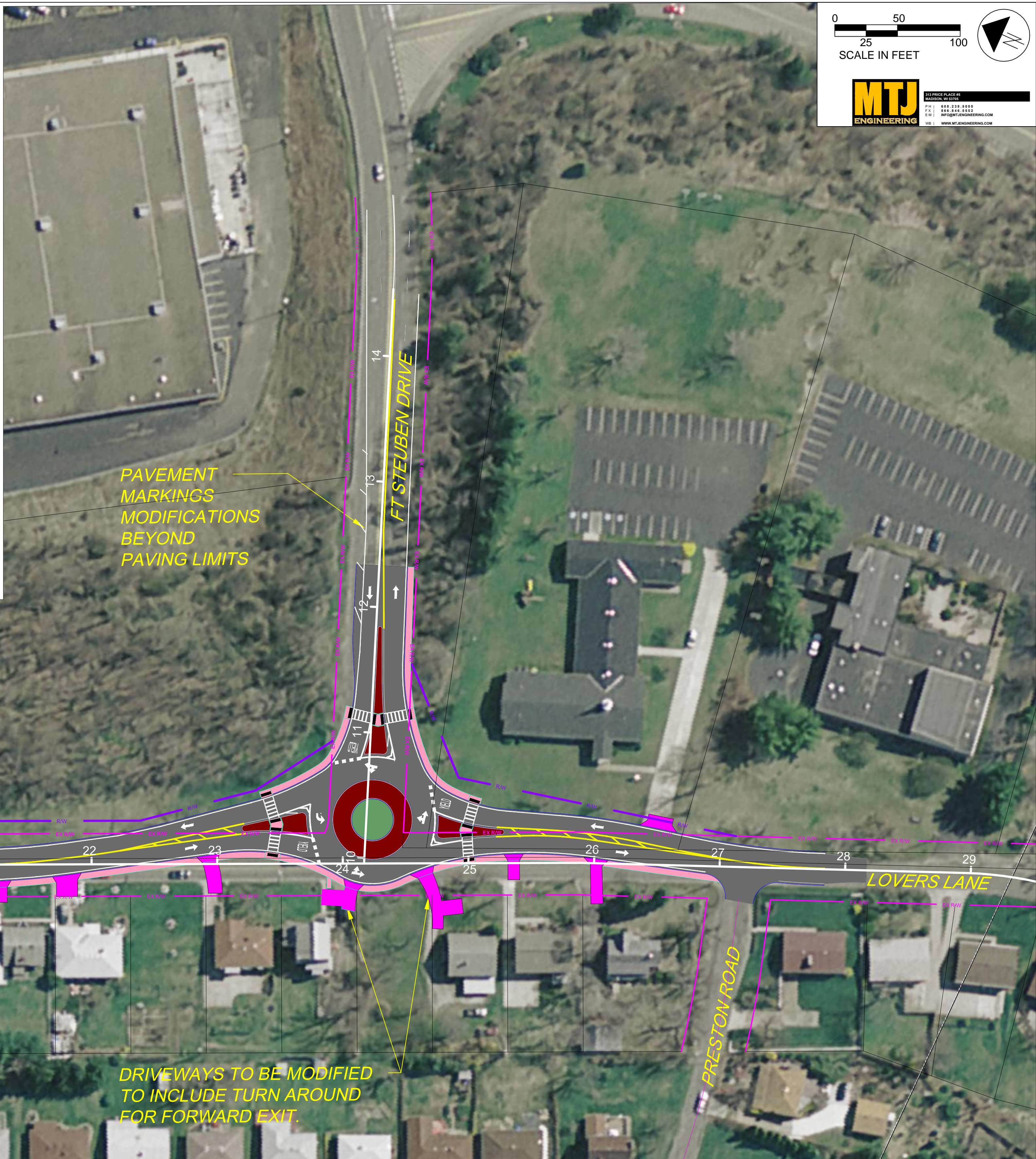
PRELIMINARY DESIGN OPTION ROUNDABOUT LOVERS LANE & FT STEUBEN DRIVE INTERSECTION
