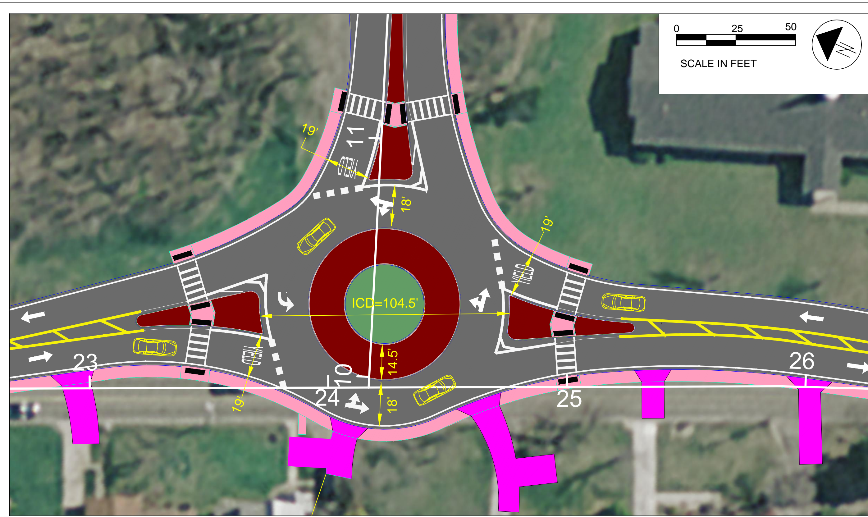
ROUNDABOUT DETAIL
